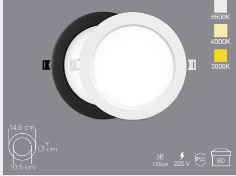
ZMR-206 18W SLIM PANEL
