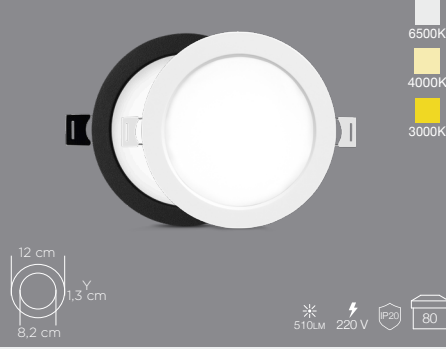
ZMR-205 15W SLIM PANEL
