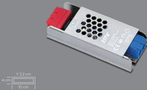
ZMR-702 12V 10A 120W SLIM LED DRIVER
