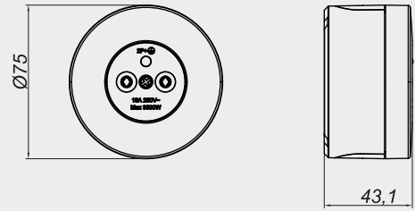
UPS PRİZ
