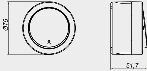
LIGHT ANAHTARI
