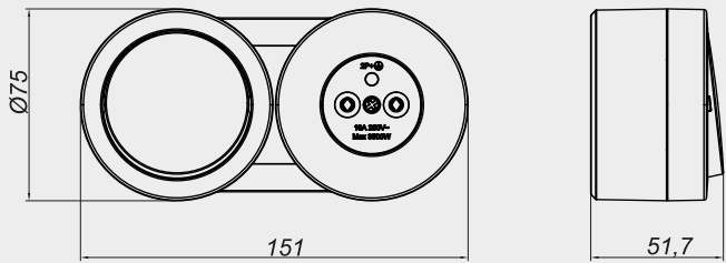
ANAHTAR + UPS PRİZ
