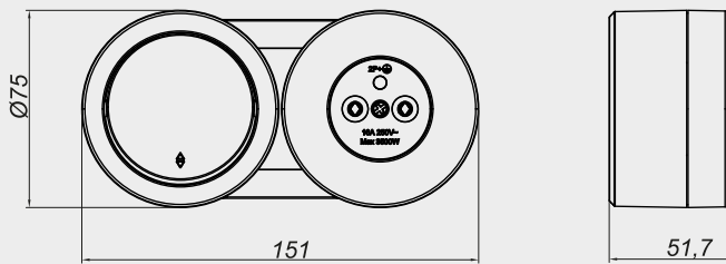
VEAVİEN + UPS PRİZ
