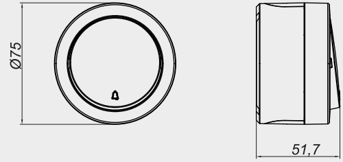
ZİL ANAHTARI
