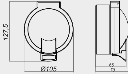
W.P. ANAHTAR
