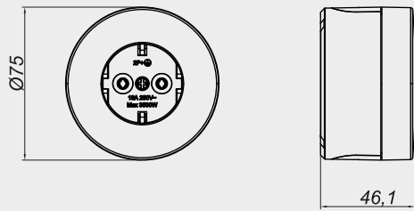
TOPRAKLI PRİZ
