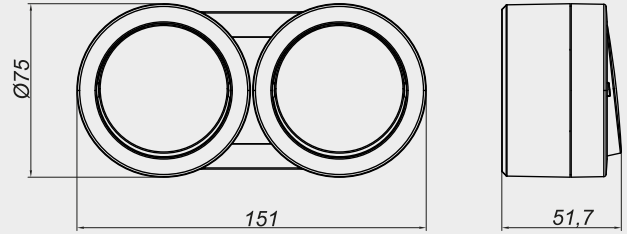
ANAHTAR + ANAHTAR
