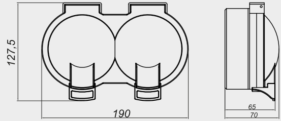
W.P. TOPRAKLI PRİZ + TOPRAKLI PRİZ
