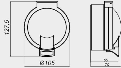
W.P. TOPRAKLI PRİZ
