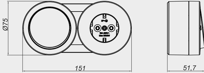
ANAHTAR + TOPRAKLI PRİZ
