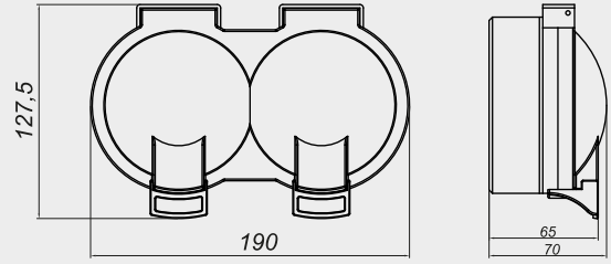
W.P. ANAHTAR + TOPRAKLI PRİZ
