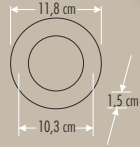
CT-5148 SLIM PANEL
