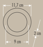
CT-5653 ZÜMRÜT BACKLIGHT PANEL
